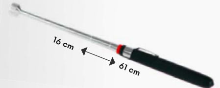
MAGNETIC TELESCOPE PICK UPPER
